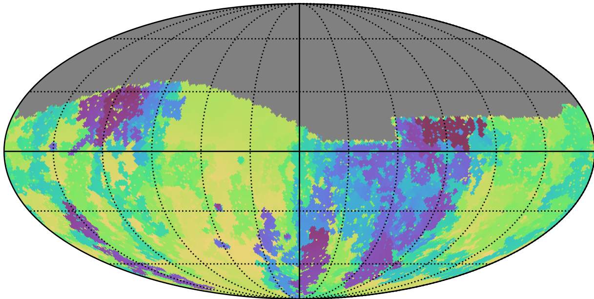
noroll_mjdp120_v3.4_10yrs Yr 1 g band: Min skyBrightness
