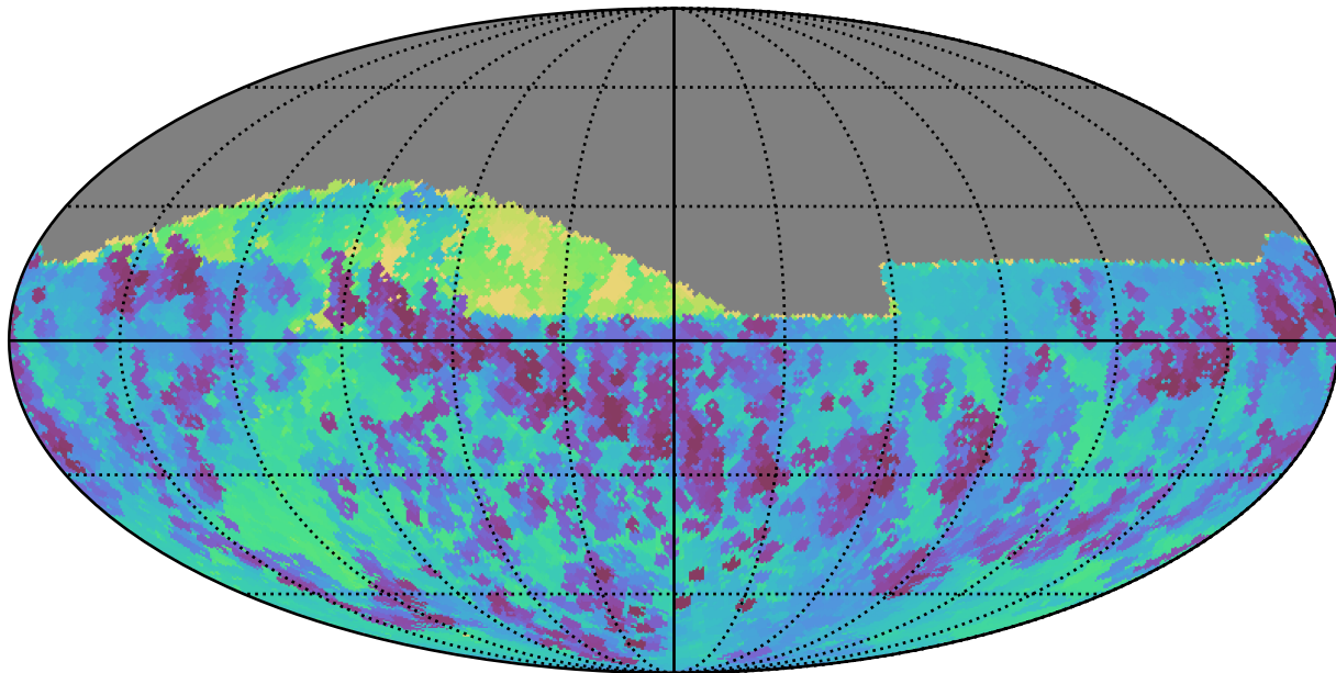
noroll_mjdp120_v3.4_10yrs Yr 1 all bands: Min skyBrightness
