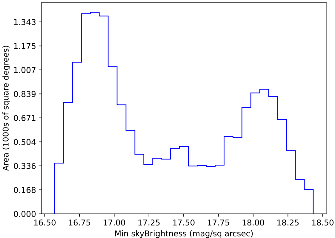
noroll_mjdp120_v3.4_10yrs WFD z band: Min skyBrightness
