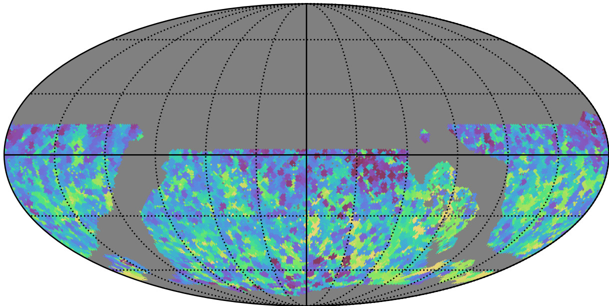
noroll_mjdp120_v3.4_10yrs WFD y band: Min skyBrightness
