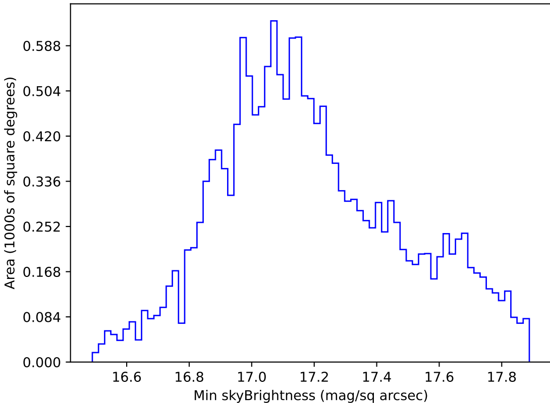
noroll_mjdp120_v3.4_10yrs WFD y band: Min skyBrightness
