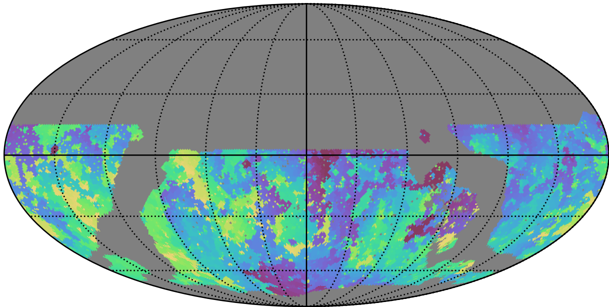
noroll_mjdp120_v3.4_10yrs WFD u band: Min skyBrightness
