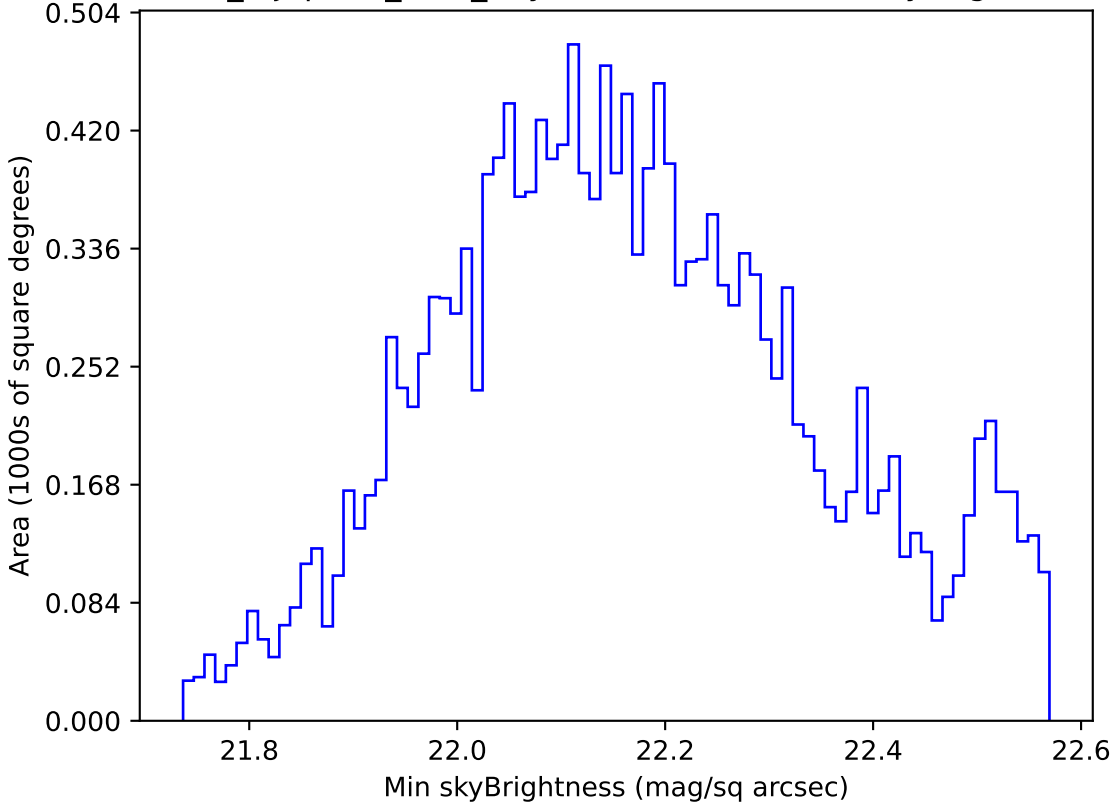
noroll_mjdp120_v3.4_10yrs WFD u band: Min skyBrightness
