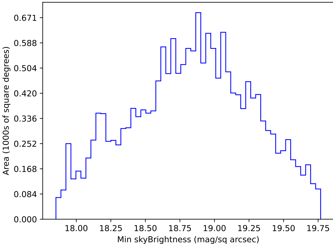
noroll_mjdp120_v3.4_10yrs WFD r band: Min skyBrightness
