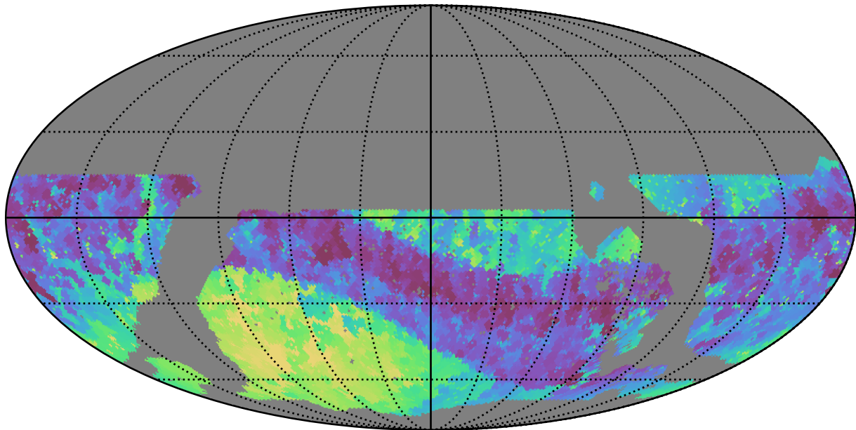
noroll_mjdp120_v3.4_10yrs WFD i band: Min skyBrightness
