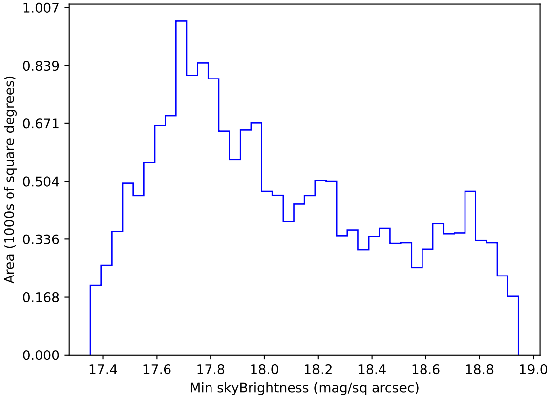
noroll_mjdp120_v3.4_10yrs WFD i band: Min skyBrightness
