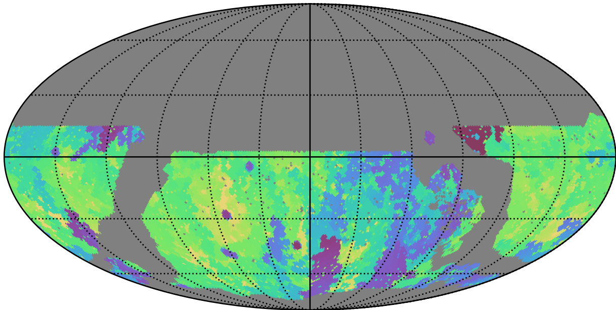
noroll_mjdp120_v3.4_10yrs WFD g band: Min skyBrightness
