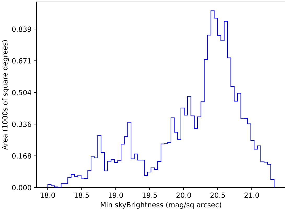
noroll_mjdp120_v3.4_10yrs WFD g band: Min skyBrightness
