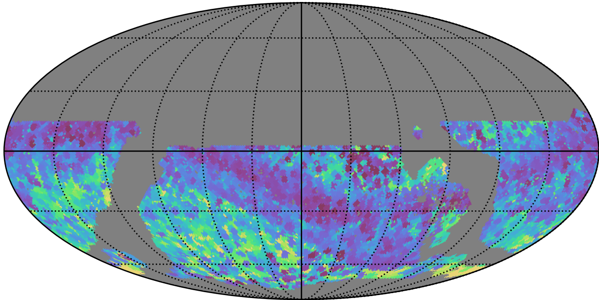
noroll_mjdp120_v3.4_10yrs WFD all bands: Min skyBrightness
