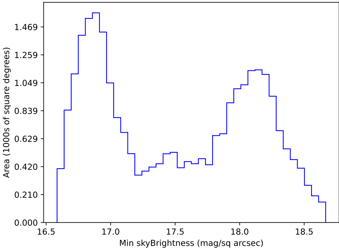
noroll_mjdp120_v3.4_10yrs All sky z band: Min skyBrightness
