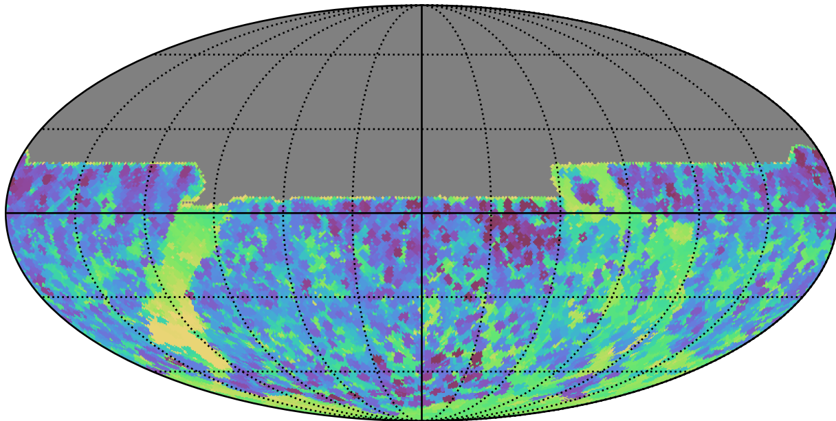
noroll_mjdp120_v3.4_10yrs All sky y band: Min skyBrightness
