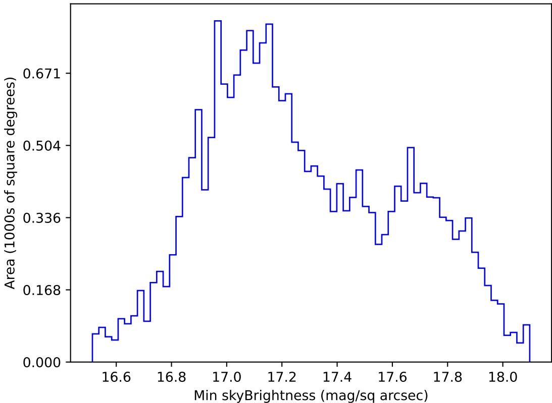
noroll_mjdp120_v3.4_10yrs All sky y band: Min skyBrightness
