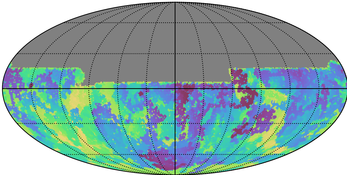
noroll_mjdp120_v3.4_10yrs All sky u band: Min skyBrightness
