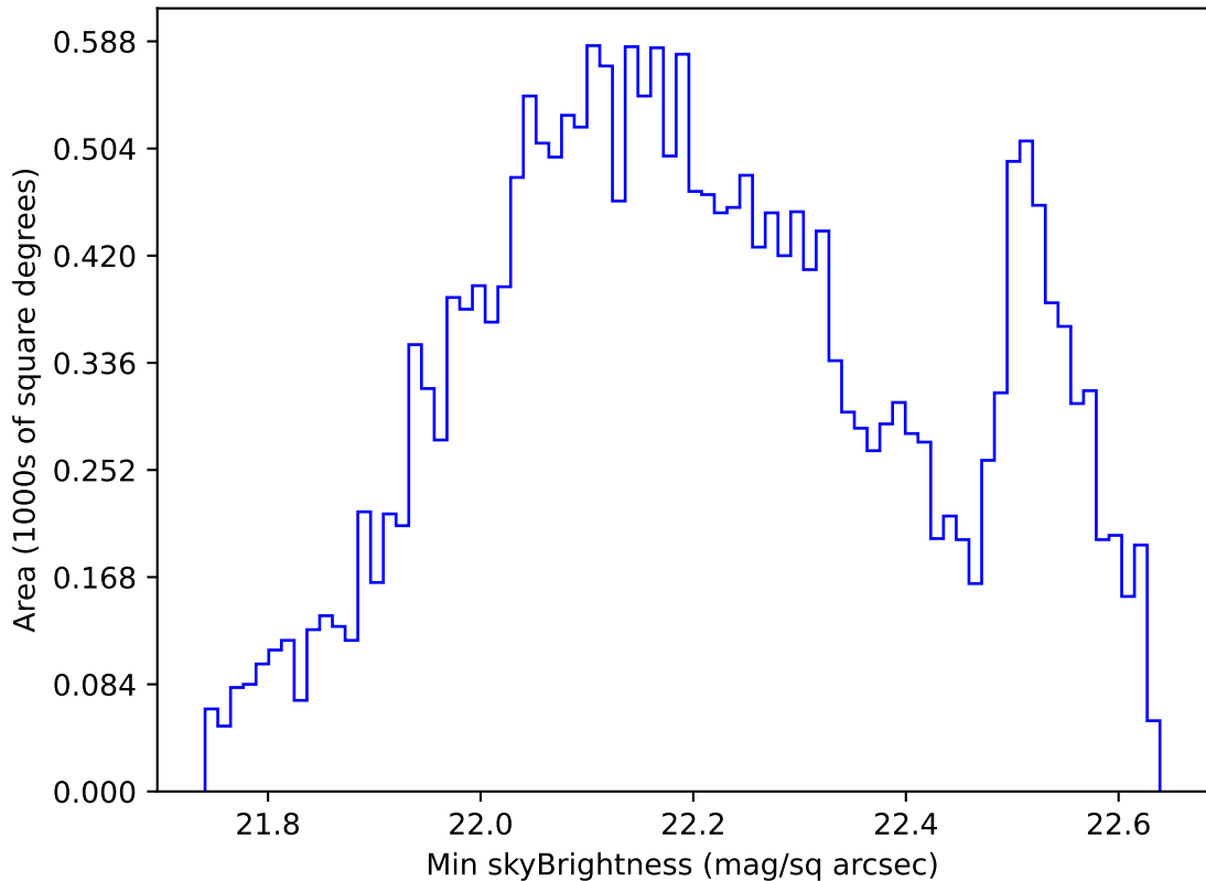
noroll_mjdp120_v3.4_10yrs All sky u band: Min skyBrightness
