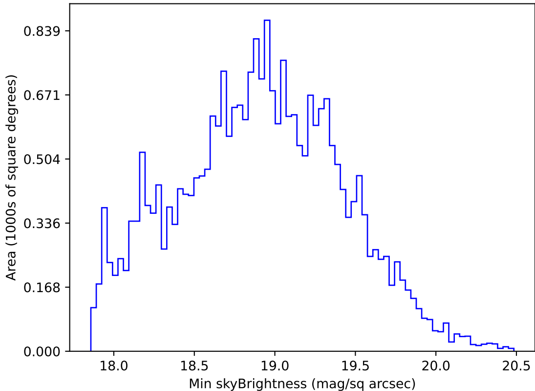
noroll_mjdp120_v3.4_10yrs All sky r band: Min skyBrightness
