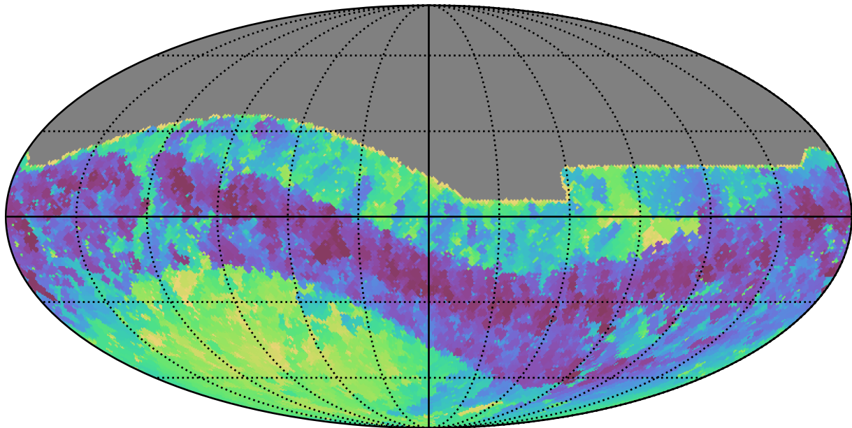
noroll_mjdp120_v3.4_10yrs All sky i band: Min skyBrightness
