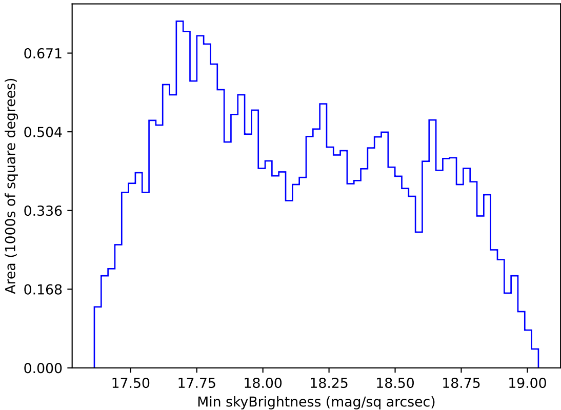
noroll_mjdp120_v3.4_10yrs All sky i band: Min skyBrightness
