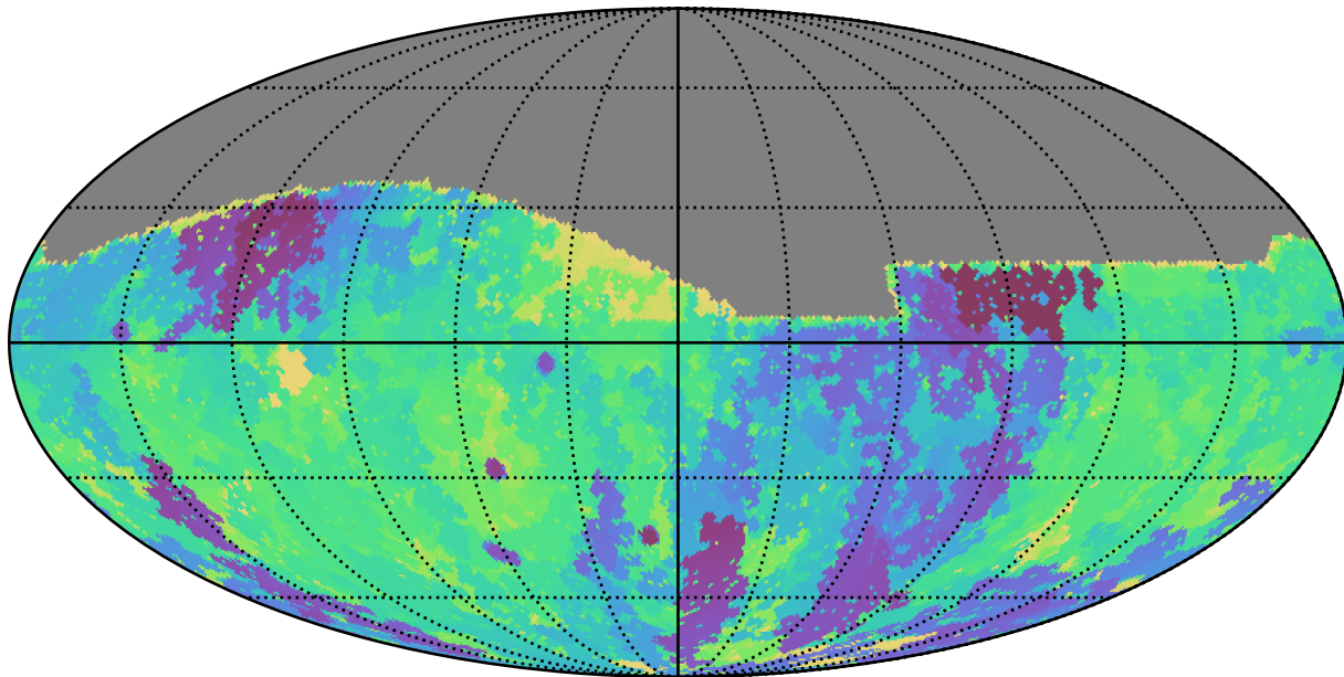
noroll_mjdp120_v3.4_10yrs All sky g band: Min skyBrightness
