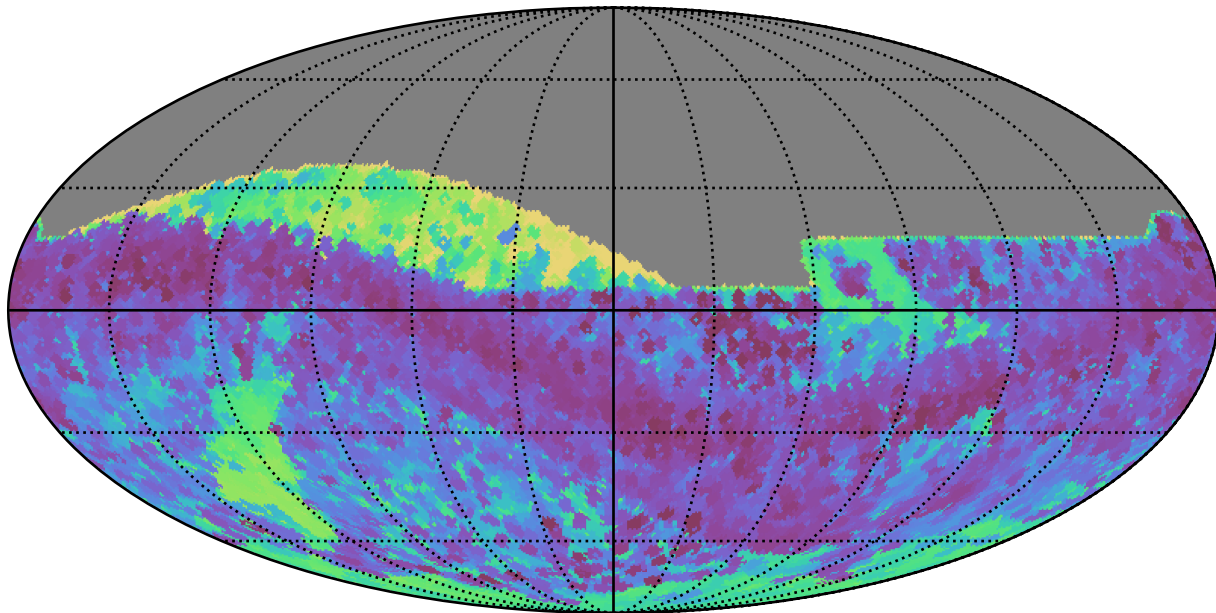
noroll_mjdp120_v3.4_10yrs All sky all bands: Min skyBrightness
