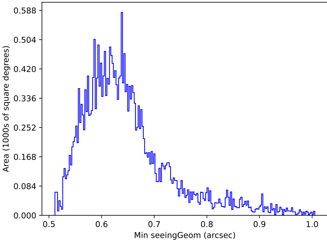
noroll_mjdp120_v3.4_10yrs Yr 1 z band: Min seeingGeom
