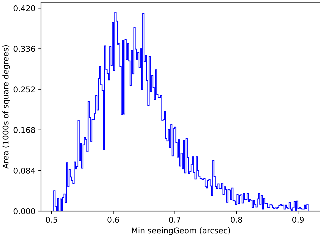
noroll_mjdp120_v3.4_10yrs Yr 1 y band: Min seeingGeom
