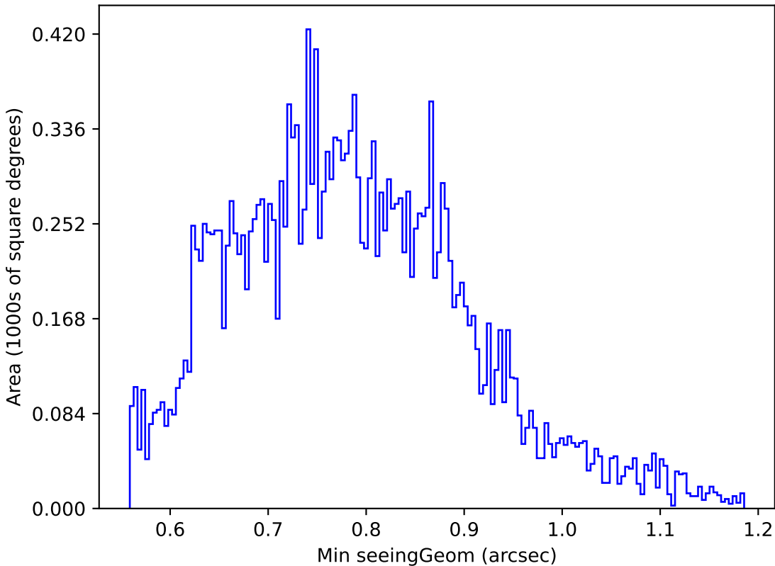
noroll_mjdp120_v3.4_10yrs Yr 1 u band: Min seeingGeom
