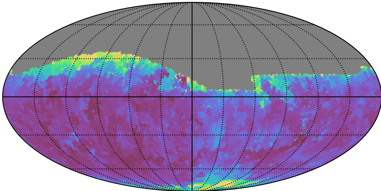
noroll_mjdp120_v3.4_10yrs Yr 1 r band: Min seeingGeom
