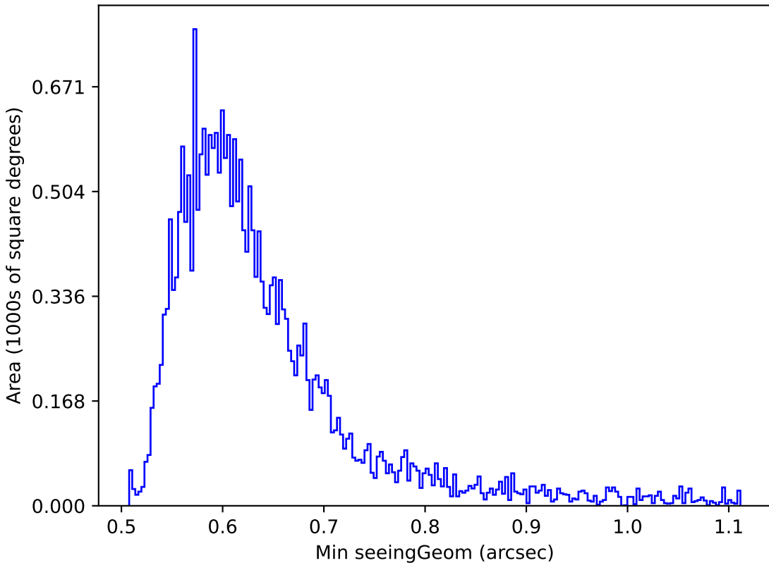
noroll_mjdp120_v3.4_10yrs Yr 1 i band: Min seeingGeom
