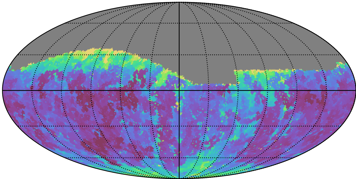
noroll_mjdp120_v3.4_10yrs Yr 1 g band: Min seeingGeom
