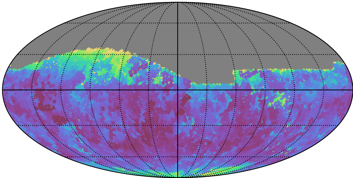
noroll_mjdp120_v3.4_10yrs Yr 1 z band: Min seeingEff
