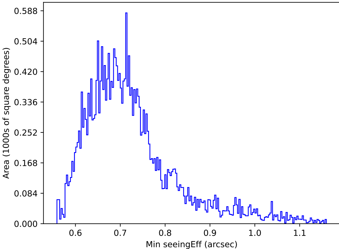
noroll_mjdp120_v3.4_10yrs Yr 1 z band: Min seeingEff
