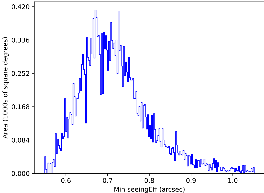
noroll_mjdp120_v3.4_10yrs Yr 1 y band: Min seeingEff
