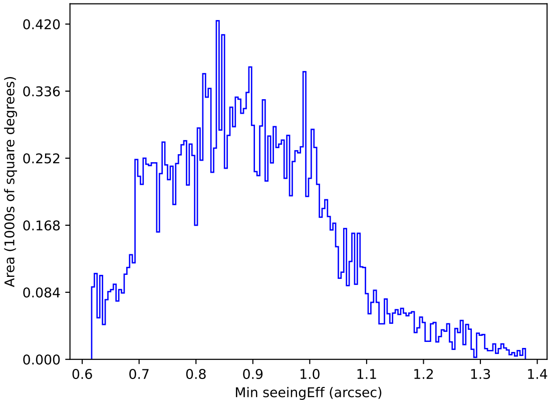
noroll_mjdp120_v3.4_10yrs Yr 1 u band: Min seeingEff
