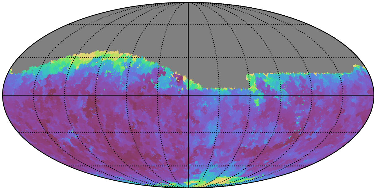
noroll_mjdp120_v3.4_10yrs Yr 1 r band: Min seeingEff
