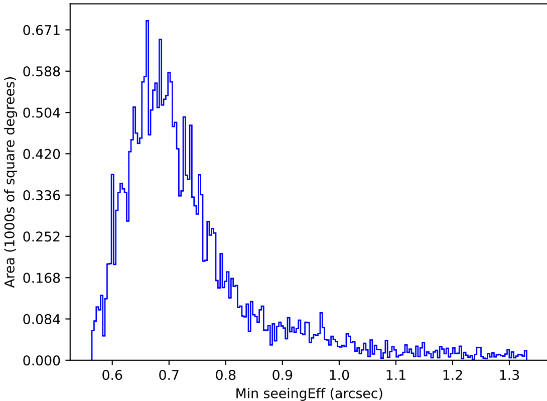
noroll_mjdp120_v3.4_10yrs Yr 1 r band: Min seeingEff
