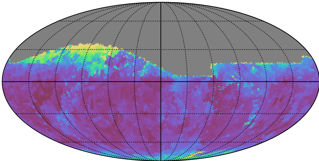
noroll_mjdp120_v3.4_10yrs Yr 1 i band: Min seeingEff
