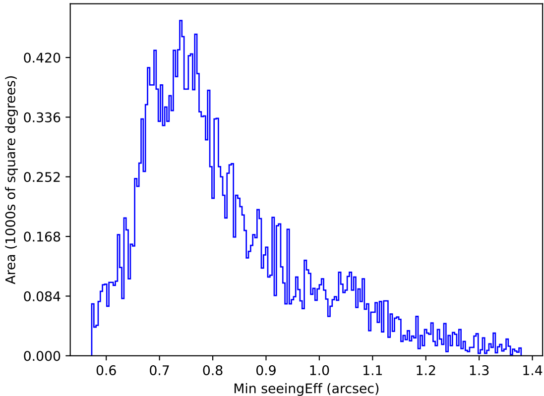
noroll_mjdp120_v3.4_10yrs Yr 1 g band: Min seeingEff
