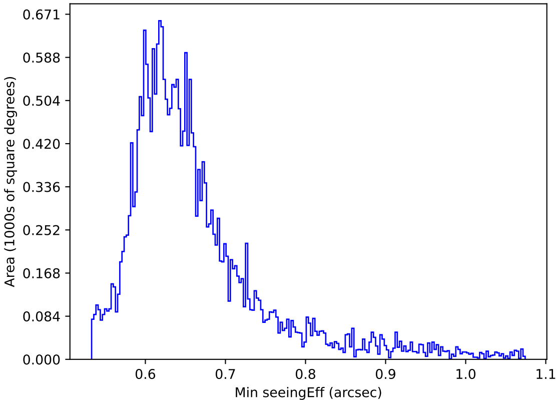
noroll_mjdp120_v3.4_10yrs Yr 1 all bands: Min seeingEff
