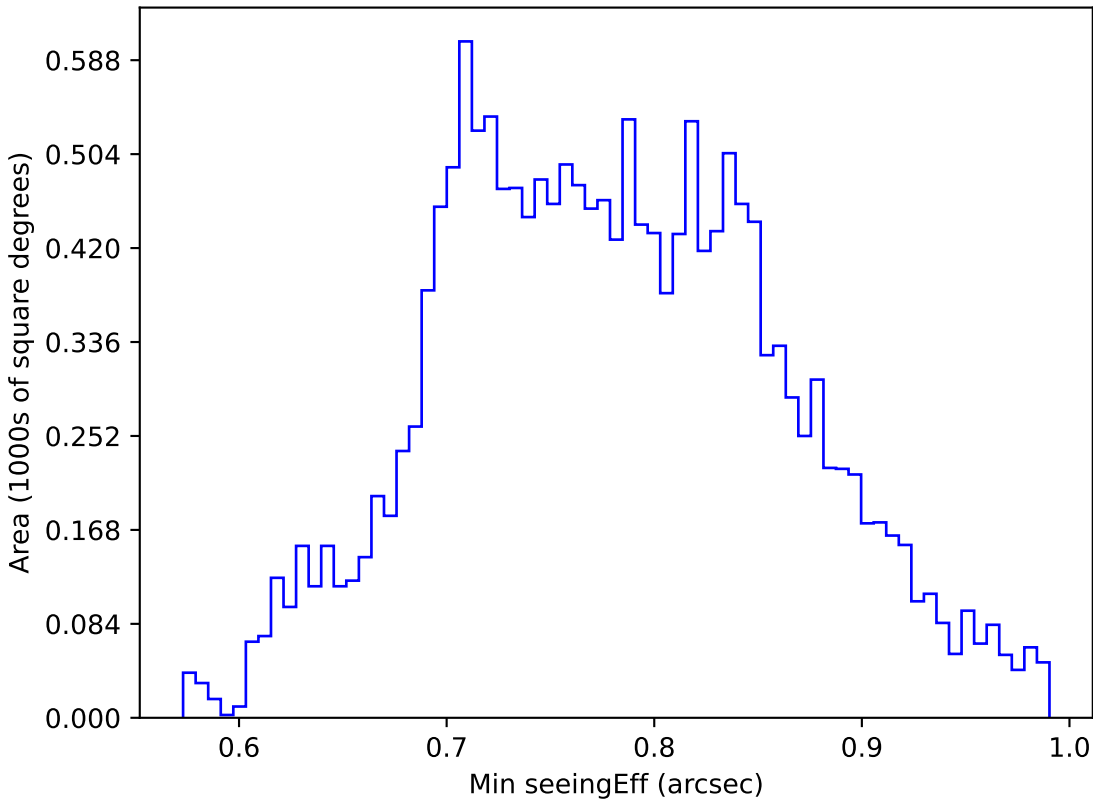
noroll_mjdp120_v3.4_10yrs WFD u band: Min seeingEff
