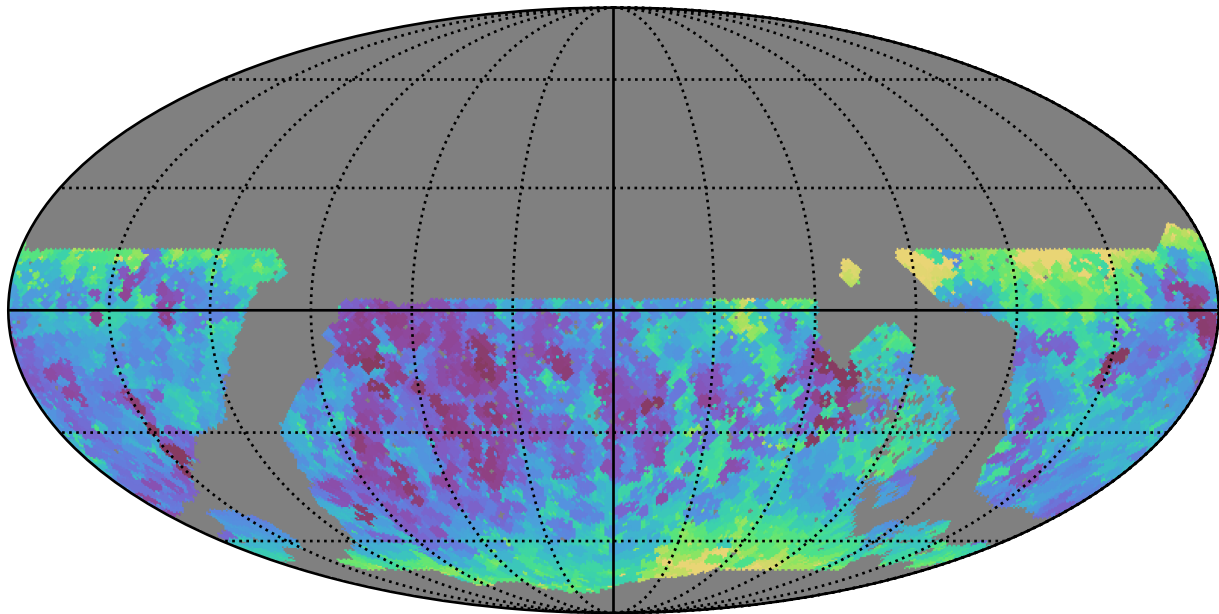
noroll_mjdp120_v3.4_10yrs WFD r band: Min seeingEff
