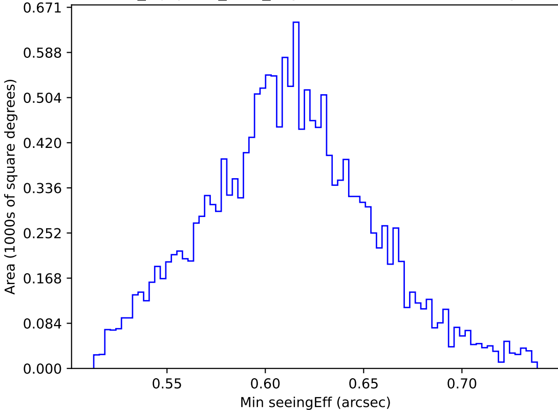
noroll_mjdp120_v3.4_10yrs WFD r band: Min seeingEff
