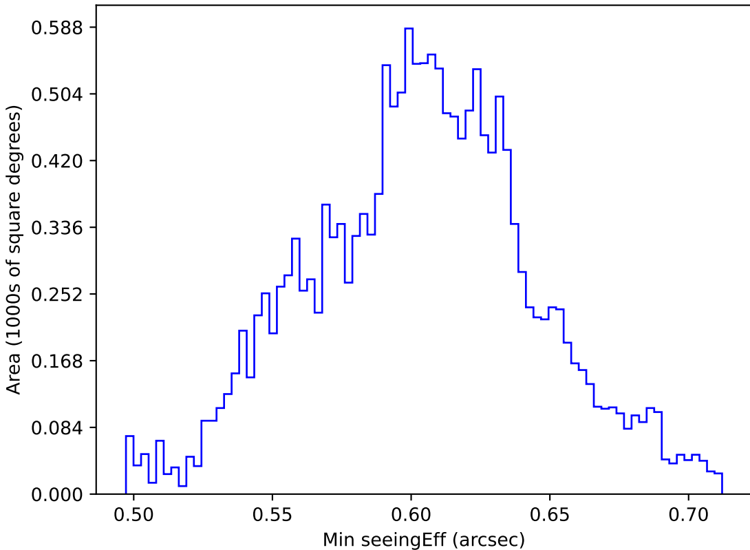
noroll_mjdp120_v3.4_10yrs WFD i band: Min seeingEff
