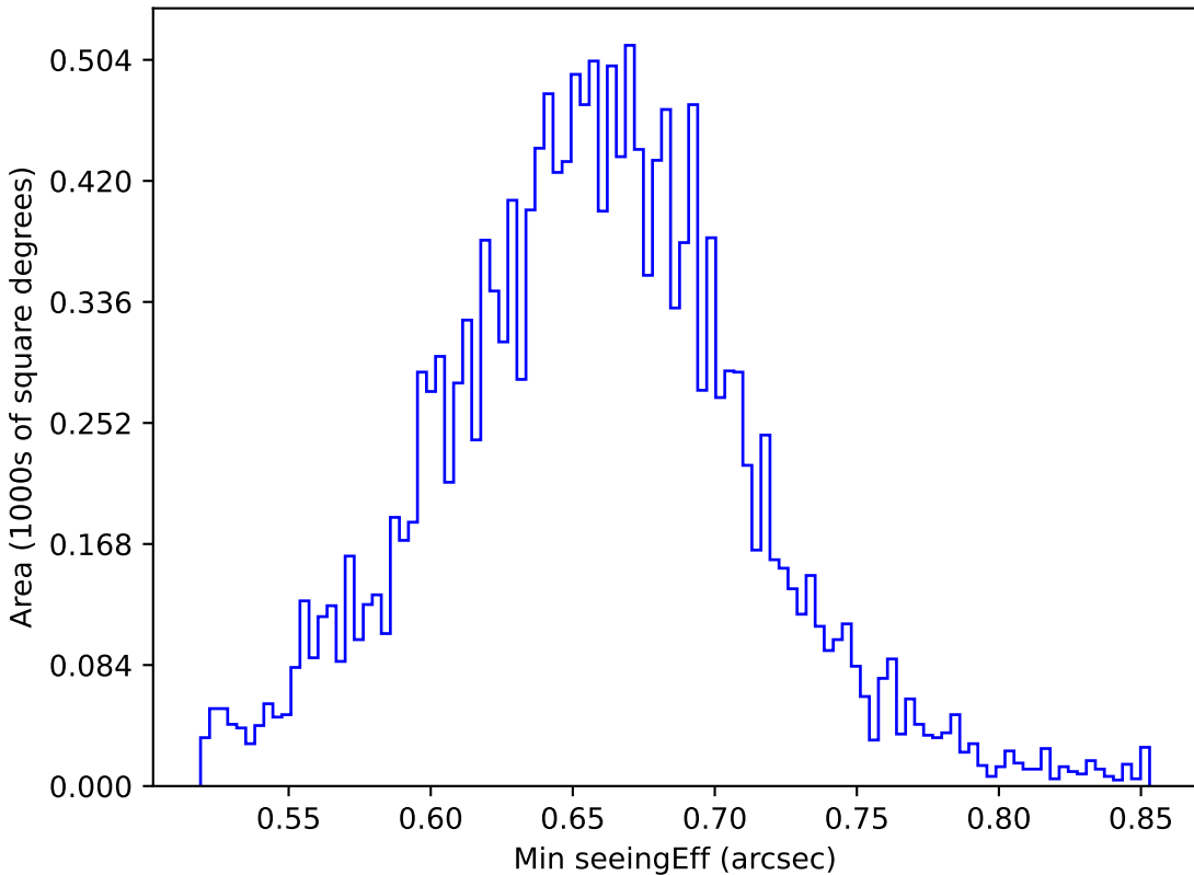
noroll_mjdp120_v3.4_10yrs WFD g band: Min seeingEff
