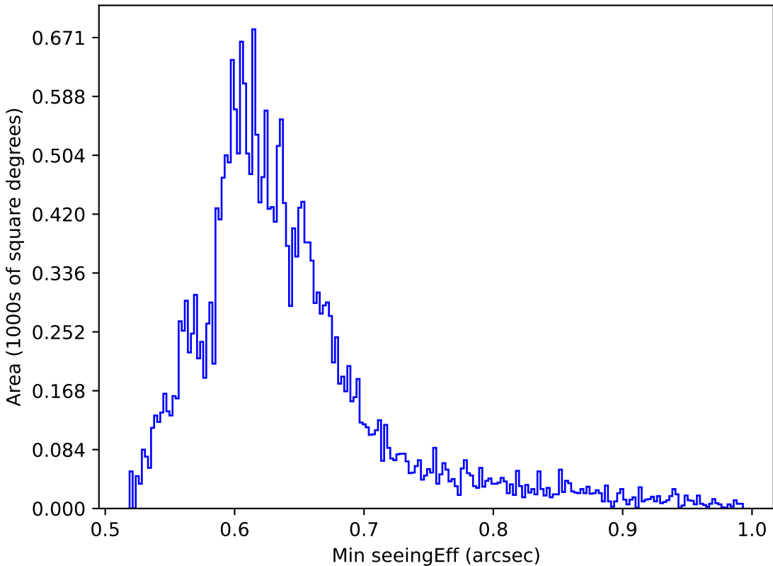
noroll_mjdp120_v3.4_10yrs All sky z band: Min seeingEff
