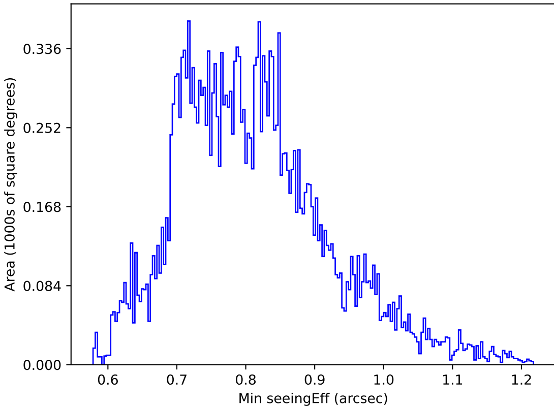
noroll_mjdp120_v3.4_10yrs All sky u band: Min seeingEff
