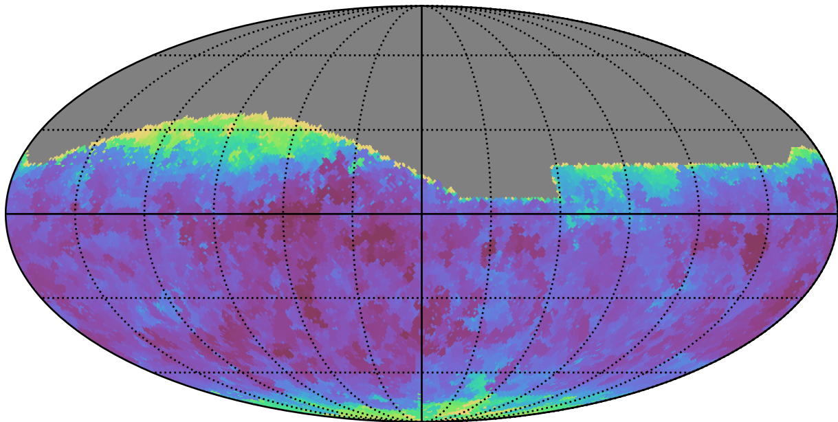
noroll_mjdp120_v3.4_10yrs All sky g band: Min seeingEff
