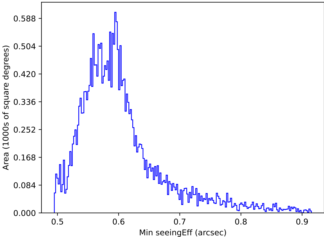
noroll_mjdp120_v3.4_10yrs All sky all bands: Min seeingEff
