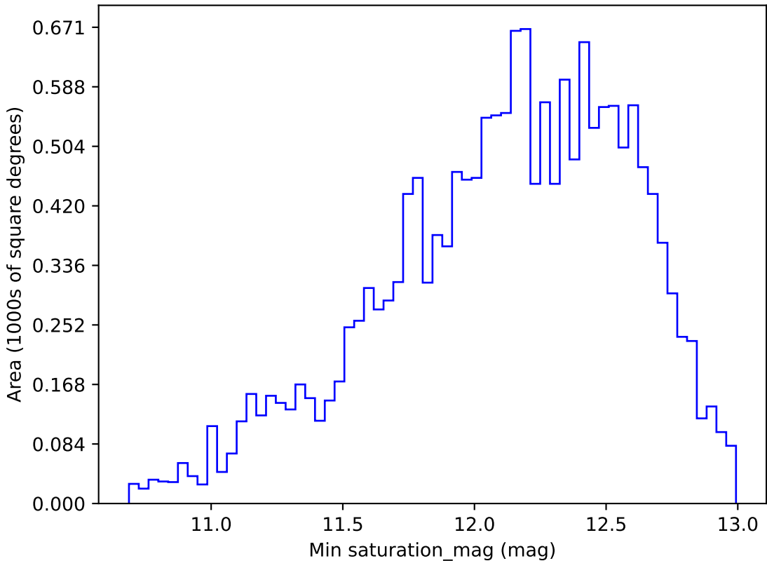
noroll_mjdp120_v3.4_10yrs WFD z band: Min saturation_mag
