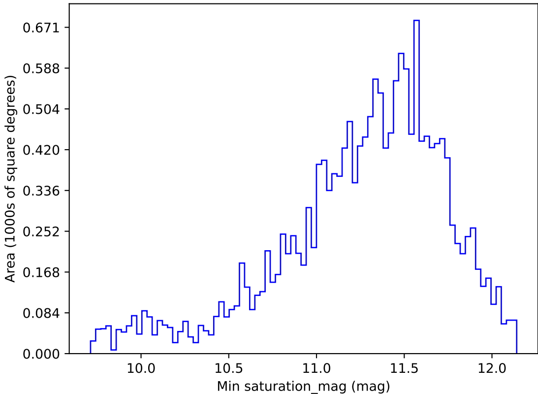
noroll_mjdp120_v3.4_10yrs WFD y band: Min saturation_mag
