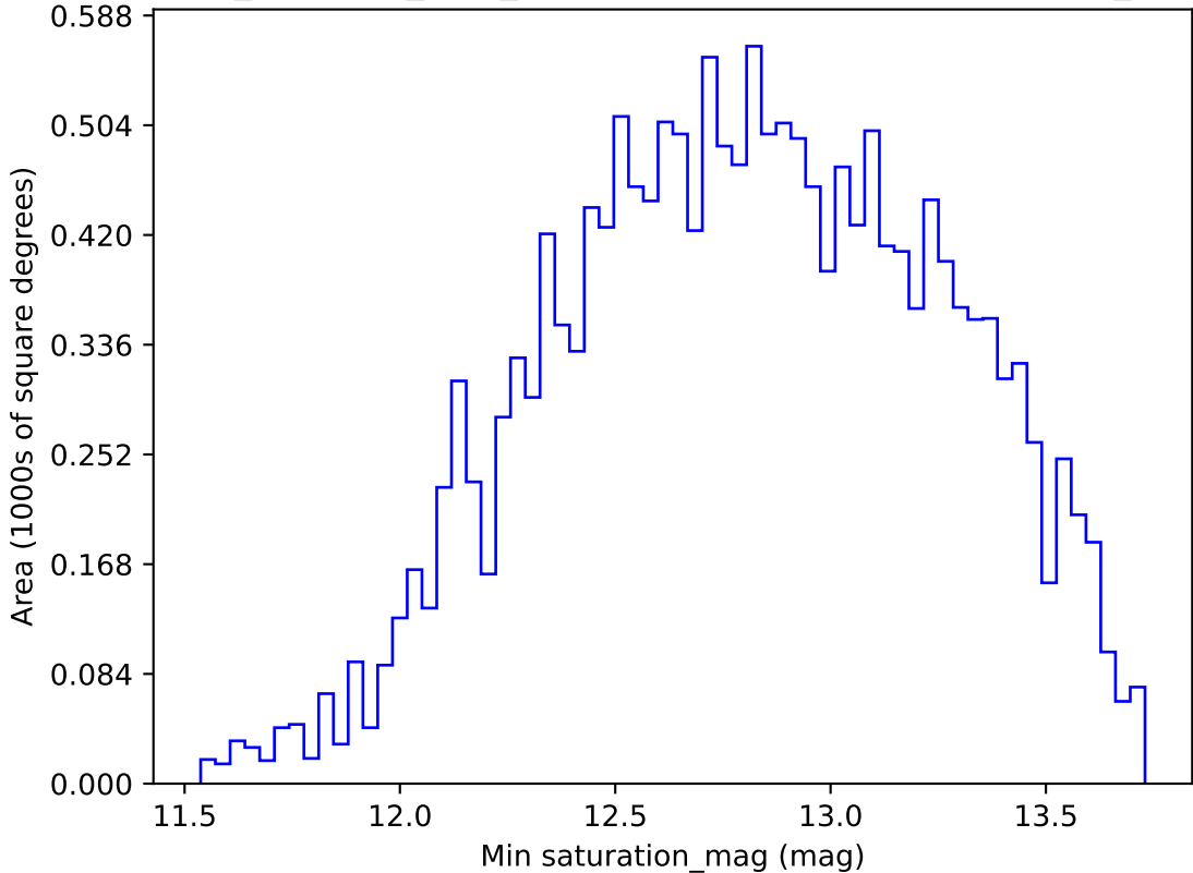
noroll_mjdp120_v3.4_10yrs WFD g band: Min saturation_mag
